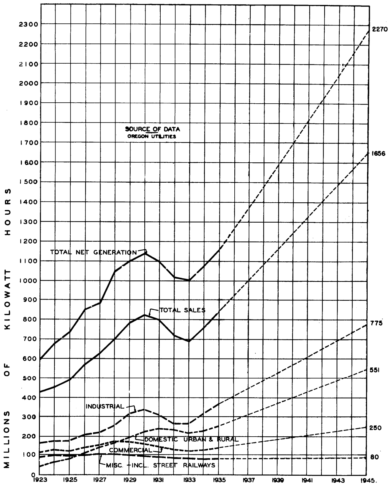
OREGON USE OF ELECTRICITY IN STATE 1923 TO 1935 INCL. WITH FORECAST OF USE TO 1945 STATE PLANNING BOARD
